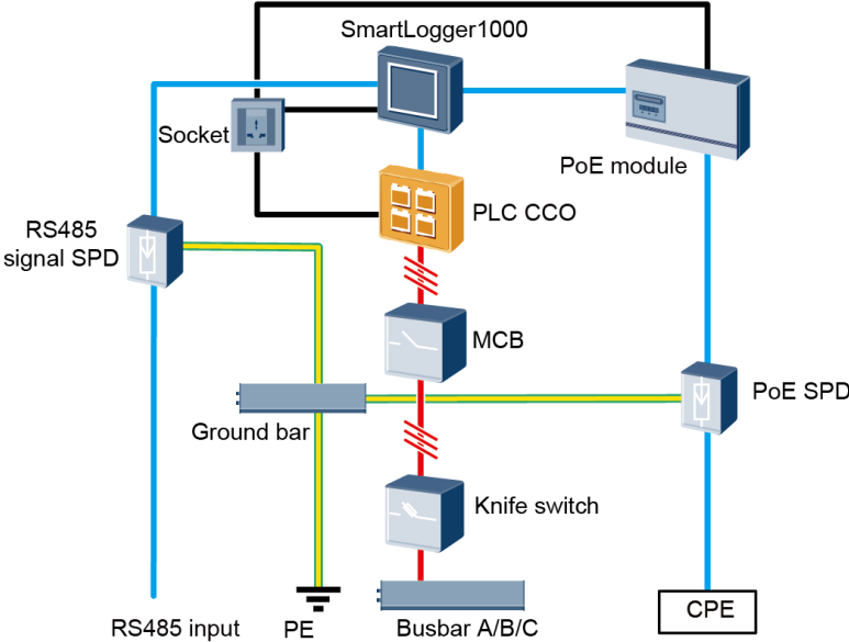
Communications cable Power cable Ground cable AC power cable — IL01110004
